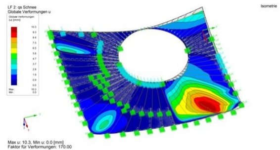
Static calculations by Timbatec
